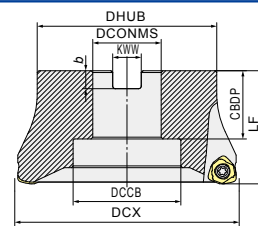
Fig.3 (エア穴無し) Without air hole
