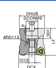
Fig.1 (エア穴付き) With air hole
